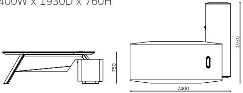
Executive Desk Item J-KR-B24L/J-KR-B24R Dimension 2400W x 1930D x 760H
